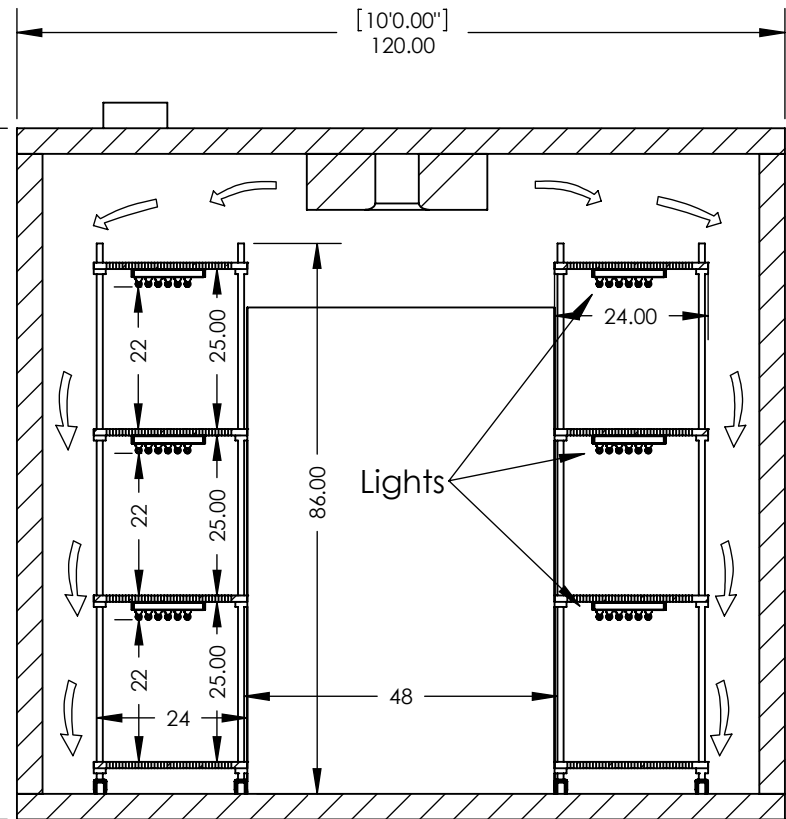
Sectional View
